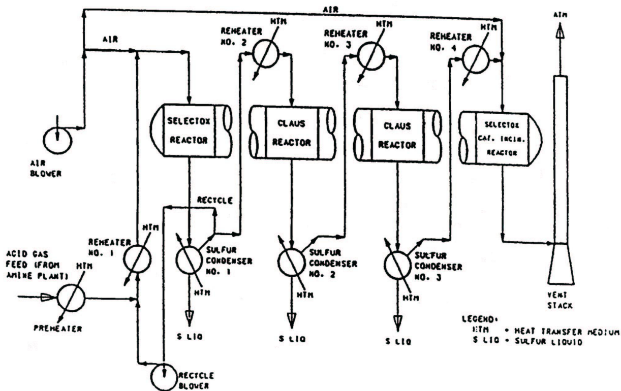
Recycle Selectox Sulfur Recovery Process (Courtesy B.G. Goar)
