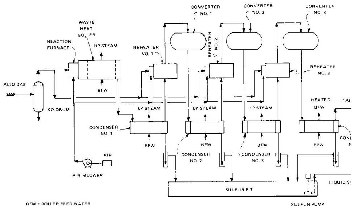
Example of Three-Stage Sulfur Plant (Straight-through operating with acid gas-fueled inline burners for reheating)
