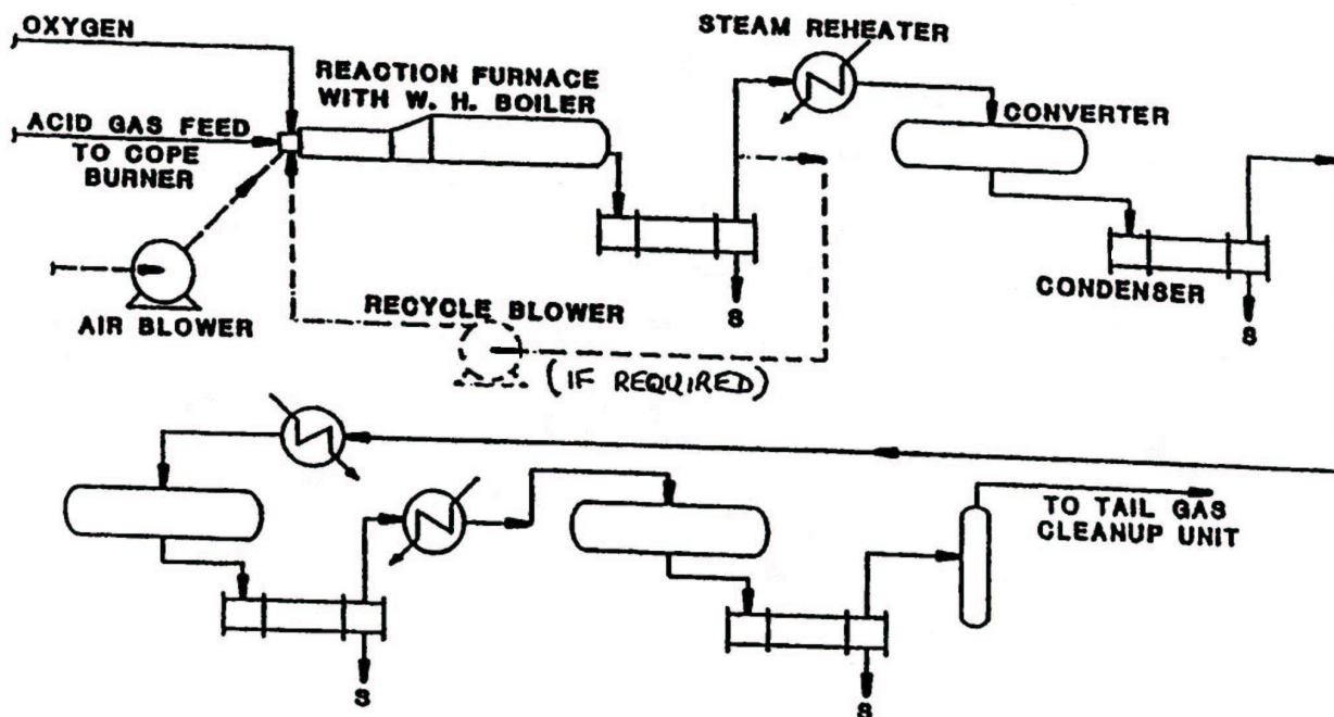
COPE SM Sulfur Recovery Unit (Courtesy Goar, Allison & Assoc.)
