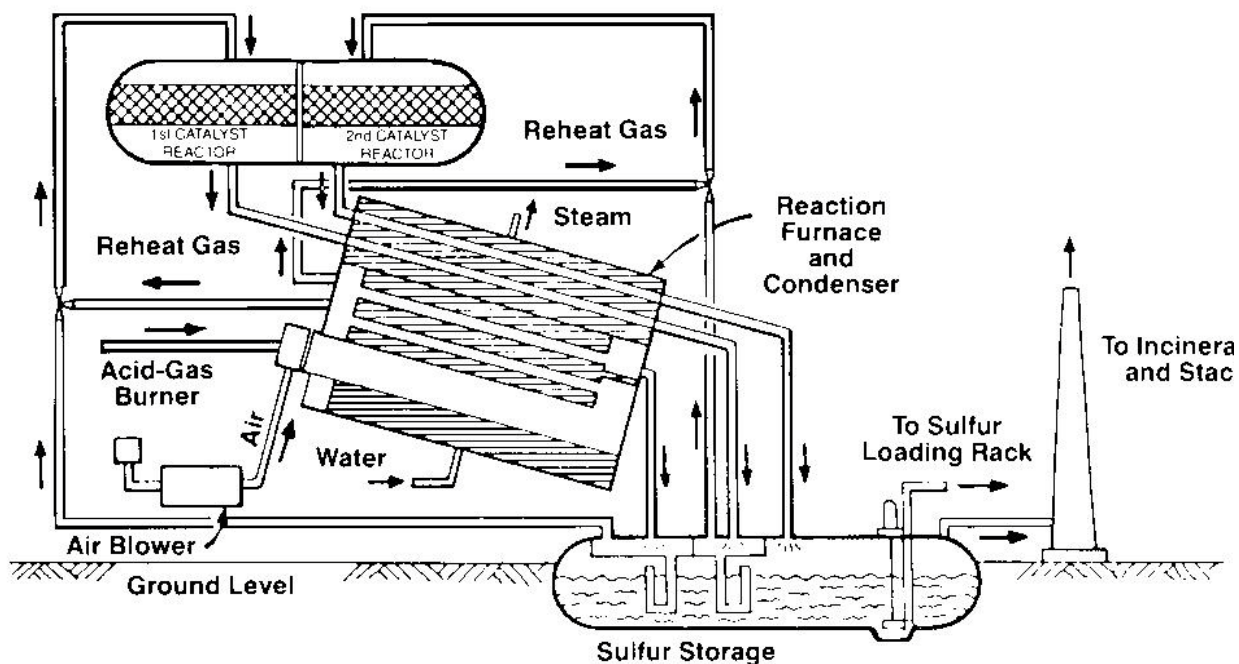
Example Package-Type Sulfur Plant
