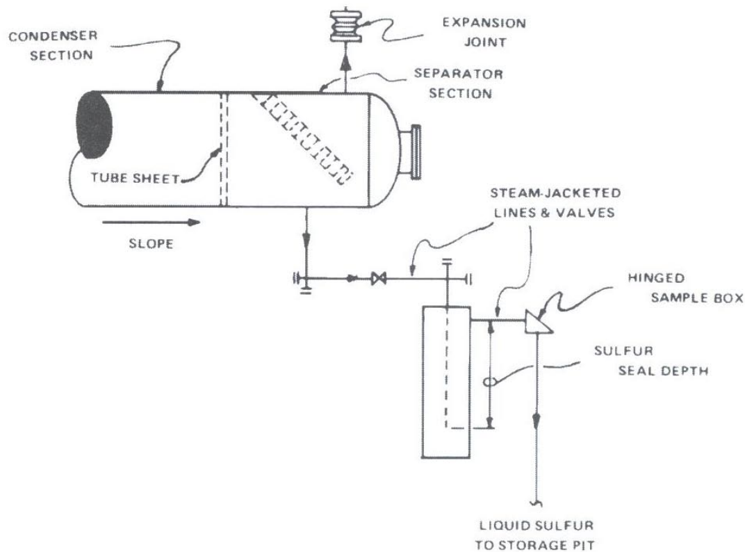
Typical Relationship of Sulfur Seal and Drain
