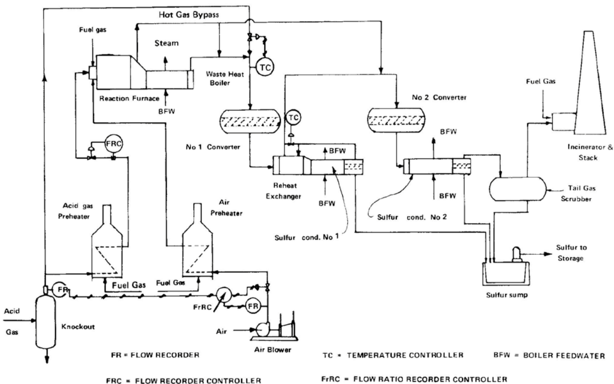
GPSA, 12 th Edition 2004 Sulfur Recovery Process with Acid Gas and Air Preheat
