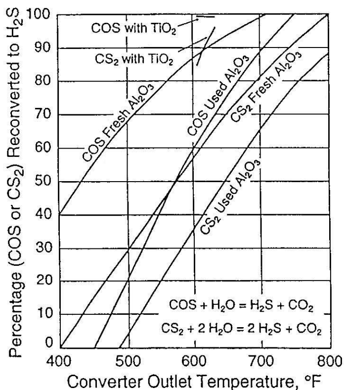
Hydrolysis of COS and CS 2 in Sulfur Converter (Reproduced from GPSSA with permission)
