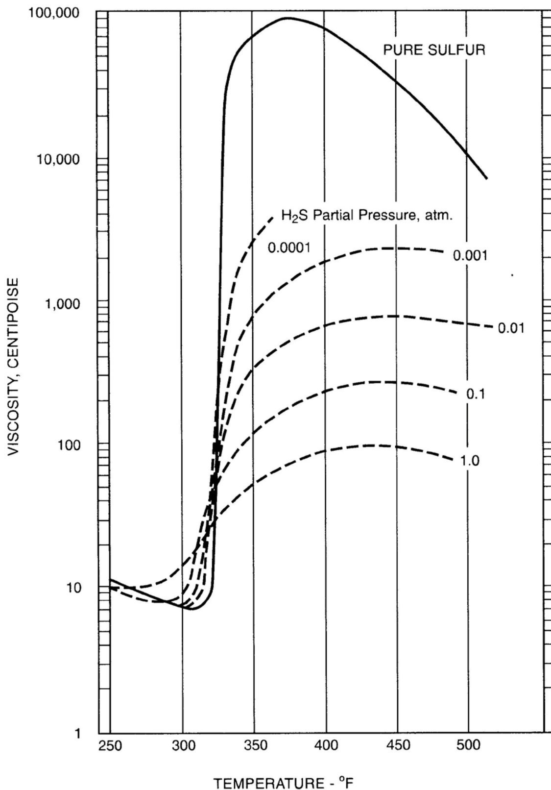
Effects of Hydrogen Sulfide on the Viscosity of Molten Sulfur
